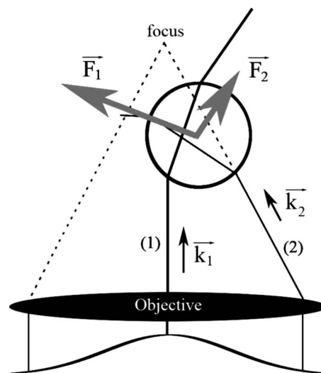
Fig. 2. Two rays (wave vectors k_1 and k_2 ) from the beam are represented, refracting at a bead localized below the focus. The rays exert forces F_1 and F_2 when refracted on the bead surface. The resulting gradient force points to the laser focus.
