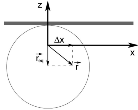
Fig. 8. Schematic of the method used to calculate F_x .
