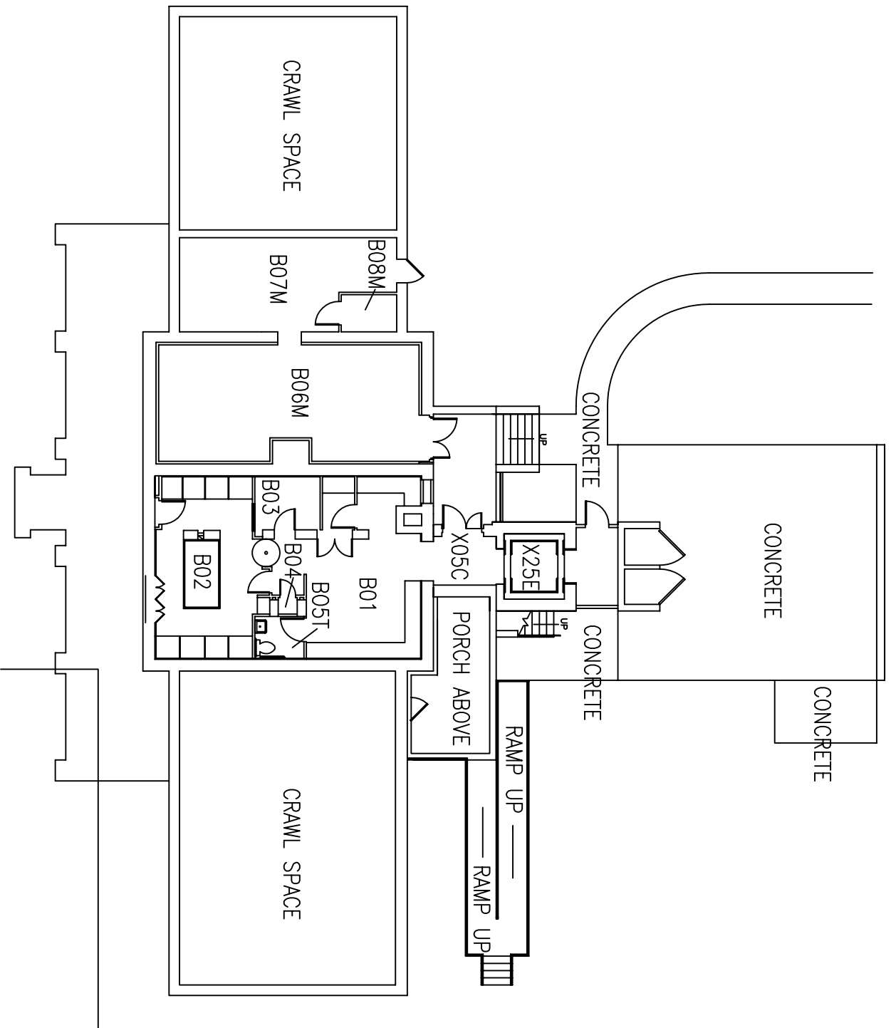
1 BASEMENT FLOOR PLAN SCALE: 1/8"=1'-0"
