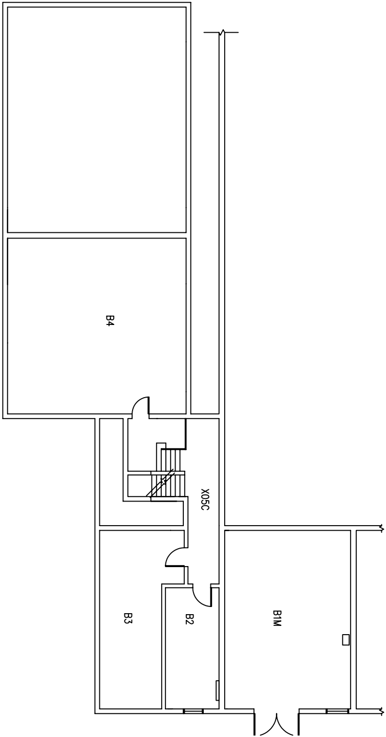
1 A1.1 BASEMENT FLOOR PLAN SCALE: 1/8"=1'-0"
