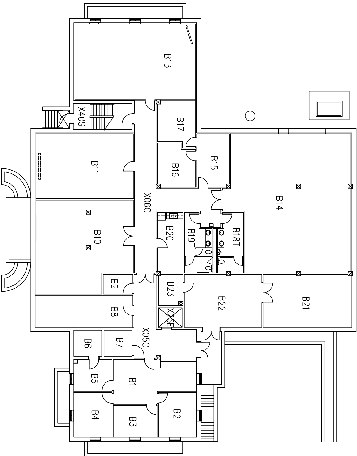
1 BASEMENT FLOOR PLAN A1.1 SCALE: 1/8"=1'-0"
