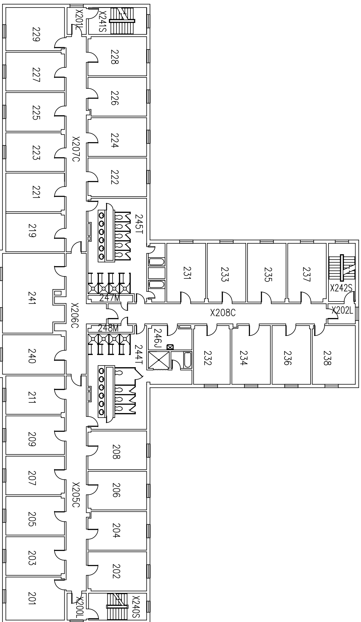
1 SECOND FLOOR PLAN A1.3 SCALE: 1/8"=1'-0"
