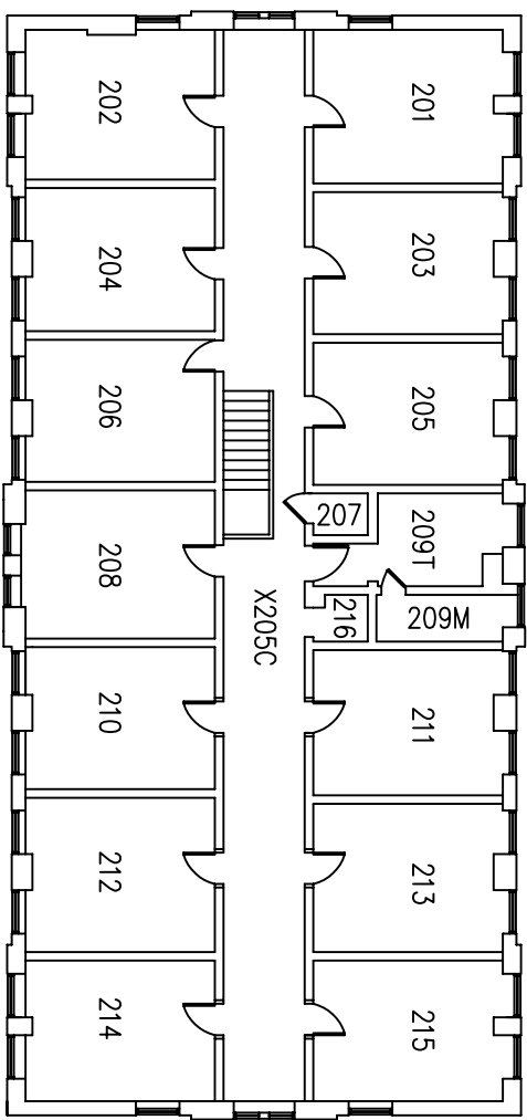
1 SECOND FLOOR PLAN A1.2 SCALE: 1/8"=1'-0"
