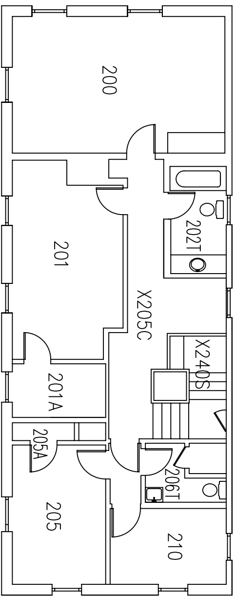
2 SECOND FLOOR PLAN A1.1 SCALE: 1/4"=1'-0"
