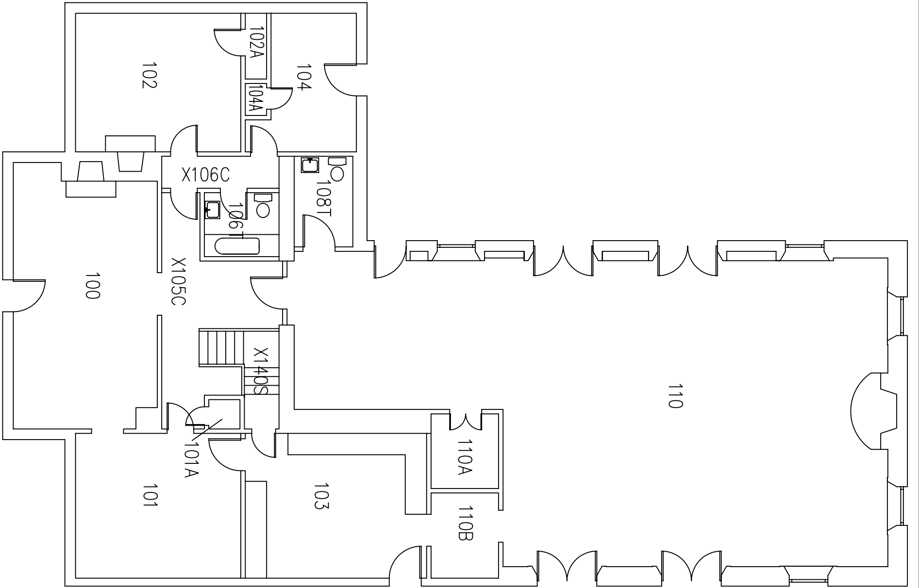
1 FIRST FLOOR PLAN A1.1 SCALE: 1/4"=1'-0"
