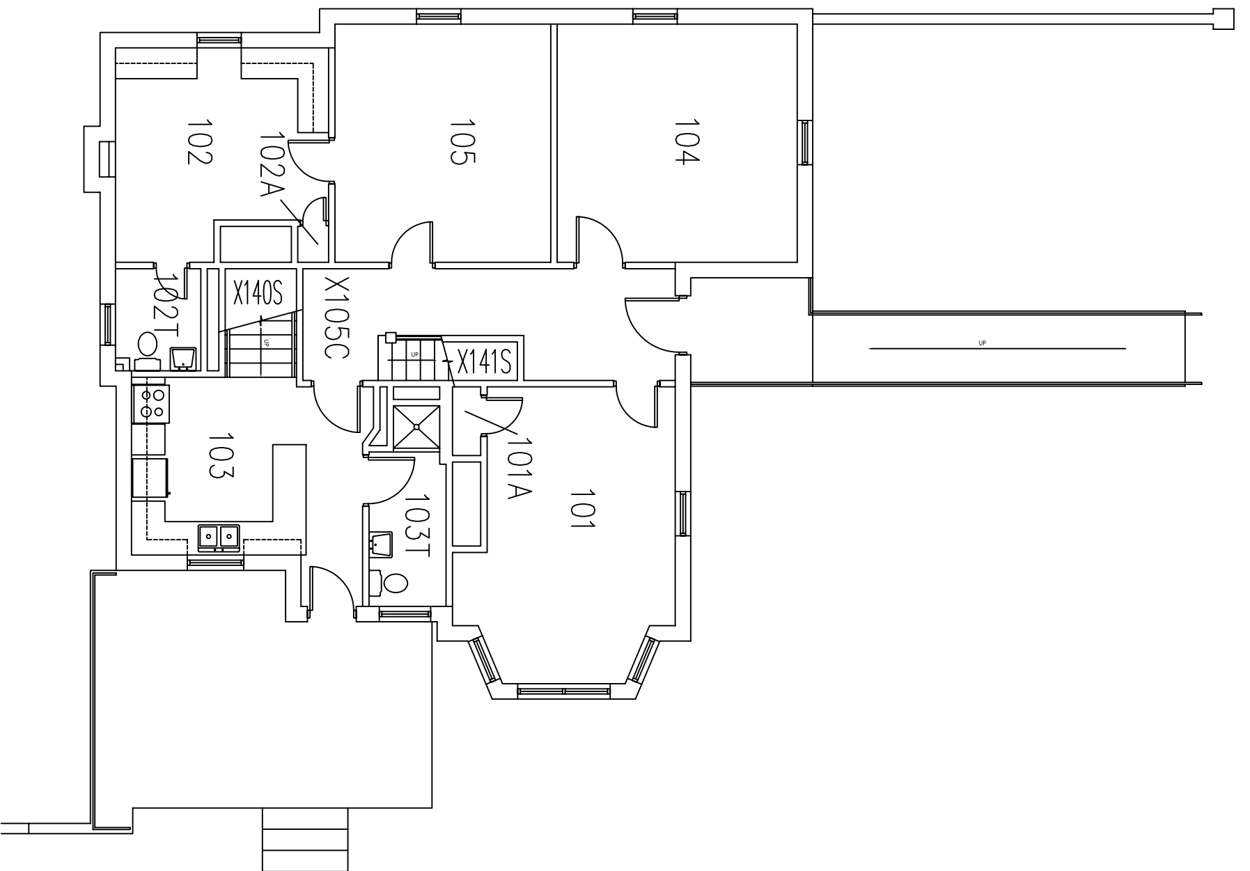
1 FIRST FLOOR PLAN A1.2 SCALE: 1/4"=1'-0"
